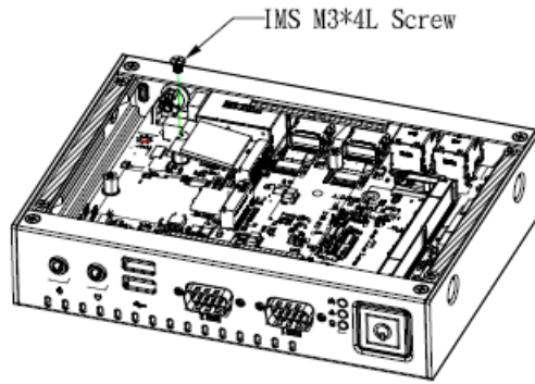
Installing M.2 Key M (2280) card
